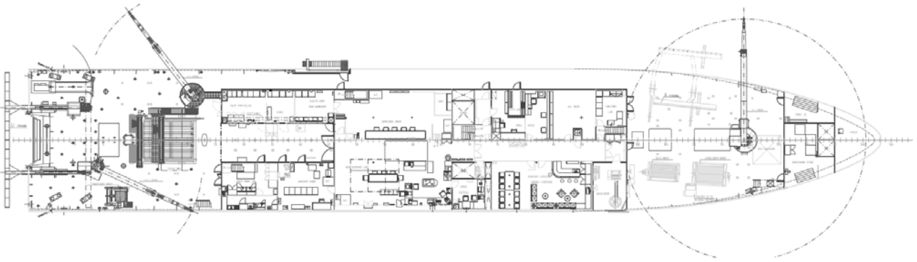
Weather Deck
