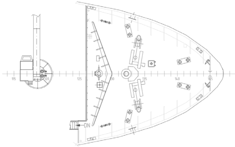
Forecastle Deck
